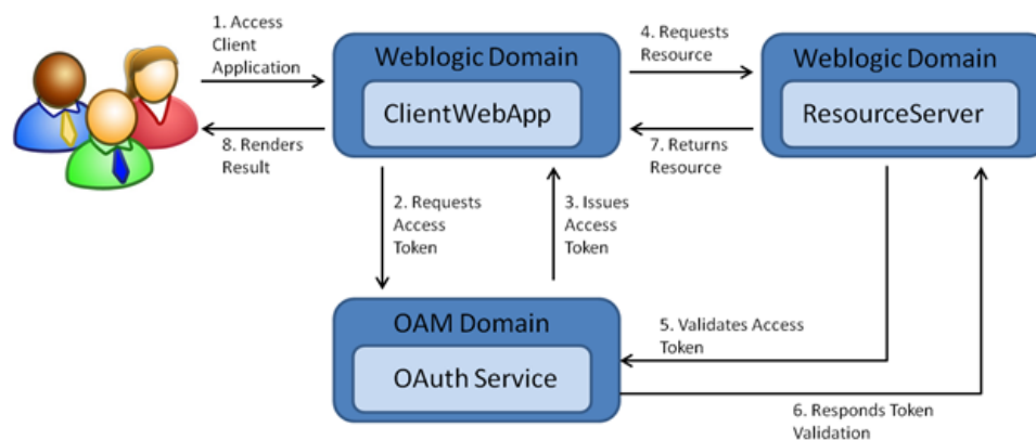
Figure 11–1 OAuth 2.0 Architecture Diagram
